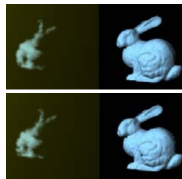
(top) 4226 64x64 maps 441 ms, 4.480 RMS error, 66.031 MB used
