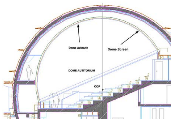
Figure 1: The Dome Theatre of FHW. 132 seats, 14.4 m dome diagonal, 20 ° of dome surface.
